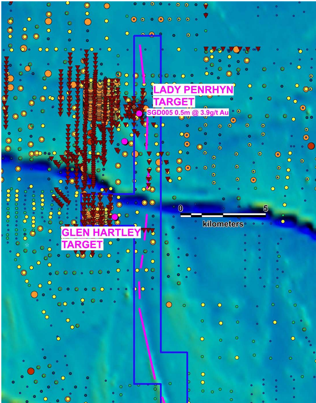
Northern Targets, Au in soils (circles), drilling (triangles). On total magnetic imagery.
